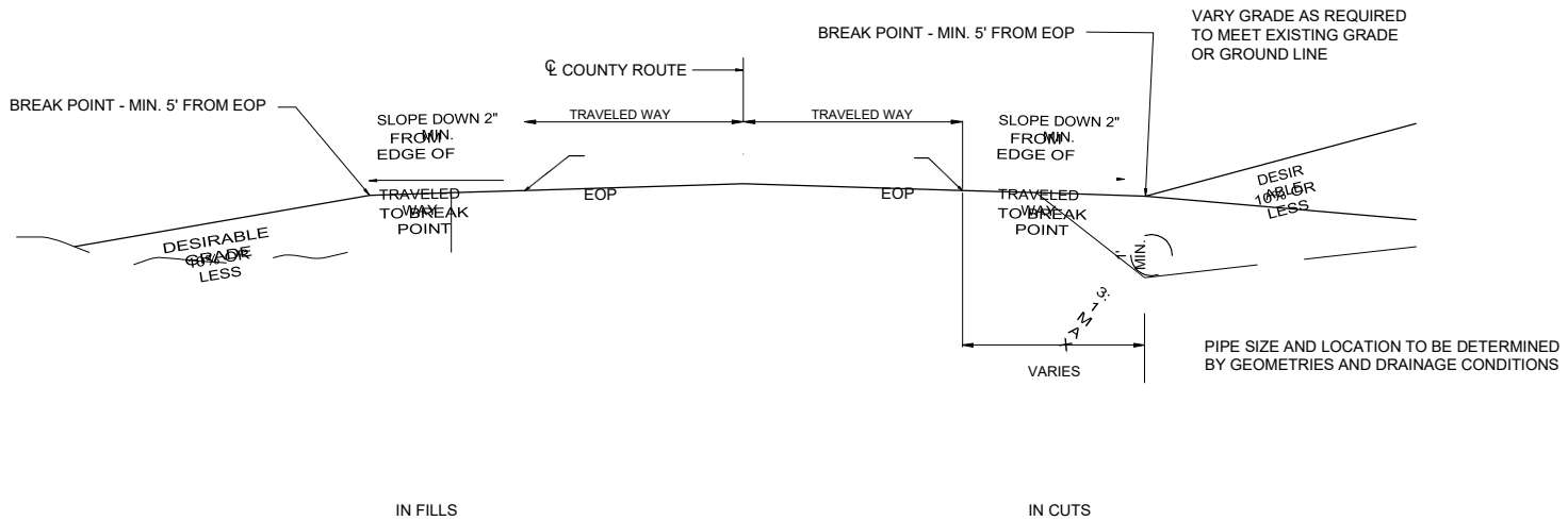
DRIVEWAY PROFILE VIEW N.T.S.
